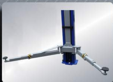
3 Stage Front Arms and 2 Stage Rear Arms
